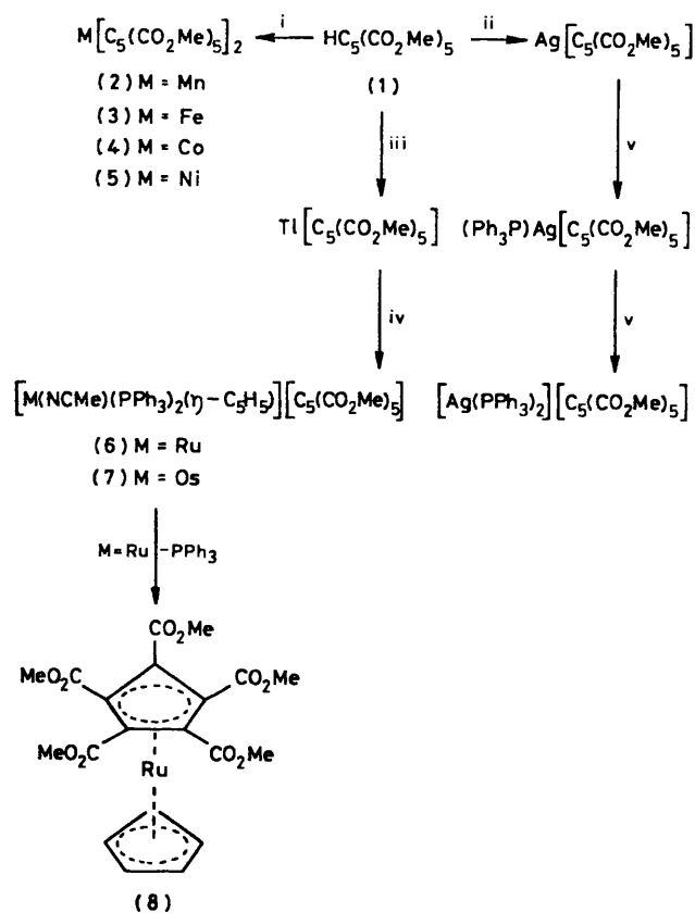
SCHEME. i, \text{M}(\text{OAc})_2 , ii, \text{AgOAc} , iii, \text{Tl}_2\text{CO}_3 , iv, \text{MCl}(\text{PPh}_3)_2(\eta\text{-C}_5\text{H}_5) in MeCN, v, \text{PPh}_3 .
